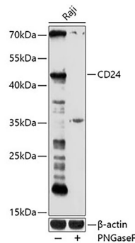
Fig. 1. Western blot analysis of extracts of Raji cells, using CD24 antibody at 1:1000 dilution. Secondary antibody: HRP-labeled Goat Anti-Rabbit IgG(H+L) (A0208) at 1:1000 dilution. Lysates/proteins: 25µg per lane. Blocking buffer: QuickBlock™ Blocking Buffer (P0231). Detection: BeyoECL Star (P0018A). Exposure time: 1s.
